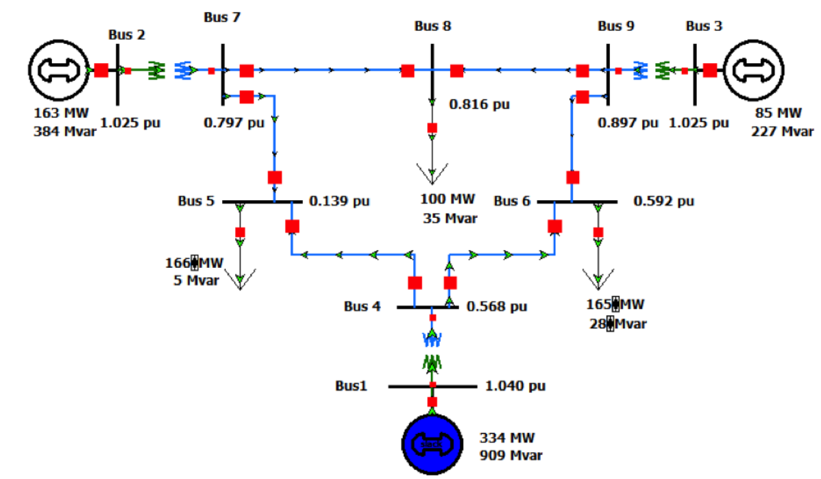
Figure 1: IEEE 9-Bus System
