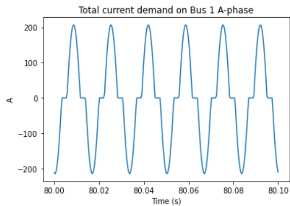
Figure 5: Total current demand on Bus 1
