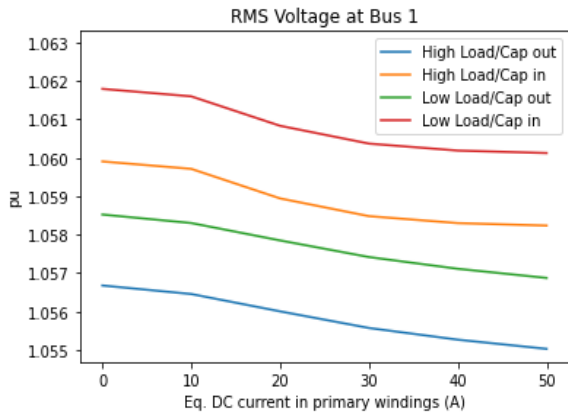
Figure 8: RMS voltage at Bus 1 against DC current magnitude for all scenarios
