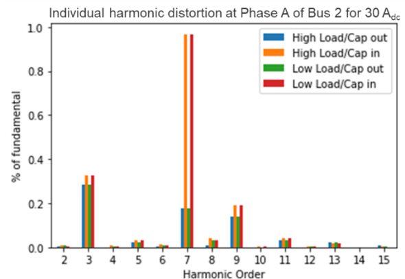
Figure 11: Individual harmonic distortion at Bus 2 for 30 A_{dc} for all tested scenarios
