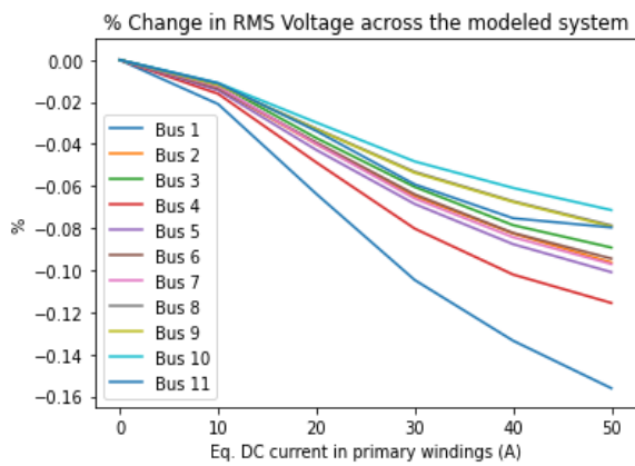
Figure 9: Percentage change in bus voltages across the system due to DC injection for the high load/cap out scenario
