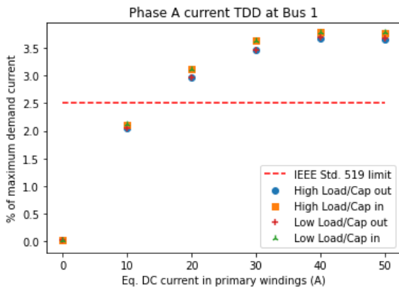
Figure 12: Current TDD at Bus 1 for all scenarios
