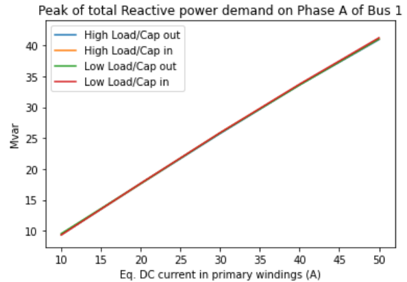
Figure 7: Q_{peak} at Phase A of Bus 1
