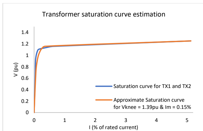
Figure 2: Comparison of measured saturation curve and approximate saturation curve corresponding to V_{knee} & I_m
