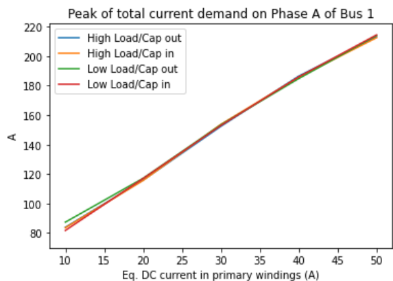
Figure 6: Peak current drawn from Bus 1 Phase A
