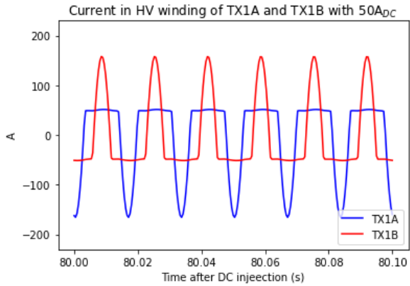
Figure 4: Primary-side currents of TX1A and TX1B
