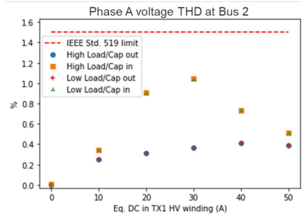
Figure 10: Voltage THD at Bus 2 for all tested scenarios
