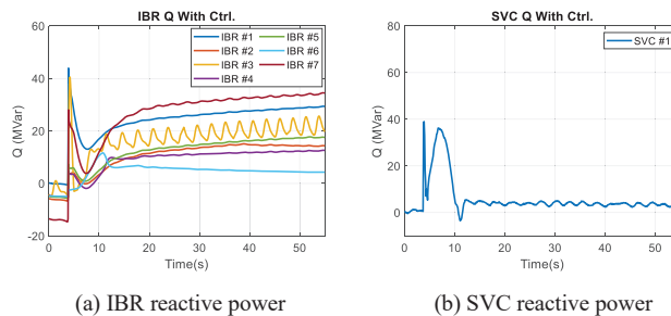
Figure 10. Reactive power of IBRs and the SVC
