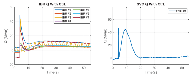
(a) IBR reactive power
