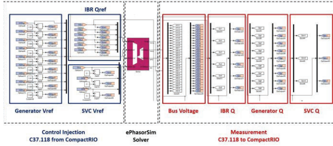
Figure 4. Implementation of the real-time simulation model
