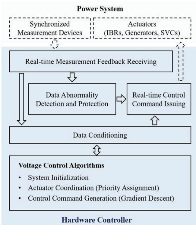
Figure 1. Structure of the hardware controller
