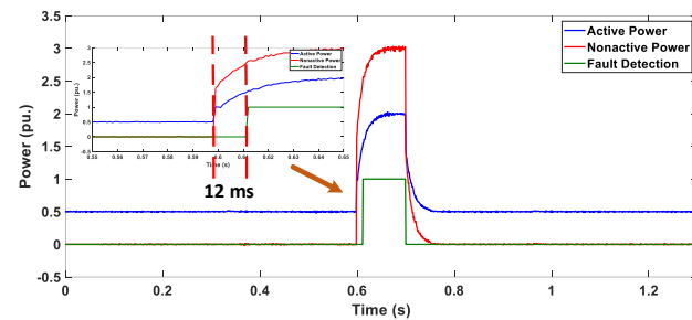
Fig. 13. BESS instantaneous power calculation and fault detection for a fault at BUS 102.
