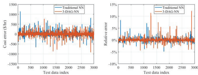
(a) Error of cost function (b) Relative error of cost function Figure 7. The error of the cost function for different NNs
