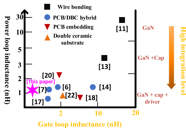
Fig. 3. Parasitic inductance and integration level of different 600 V and 650 V GaN power modules.
