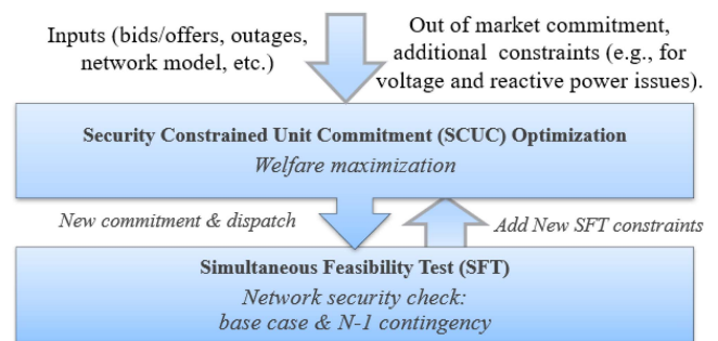
Fig. 1. SCUC and SFT iteration for market clearing.
