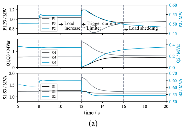
Fig. 13. Performance of current limiter in Scenario 2-1 (a) dynamic inverter output; (b) static inverter output; (c) dynamic freq. & voltage.
