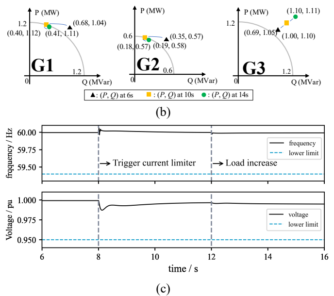
Fig. 11. Performance of proposed control framework in Scenario 2: (a) dynamic inverter output; (b) static inverter output; (c) dynamic frequency and voltage
