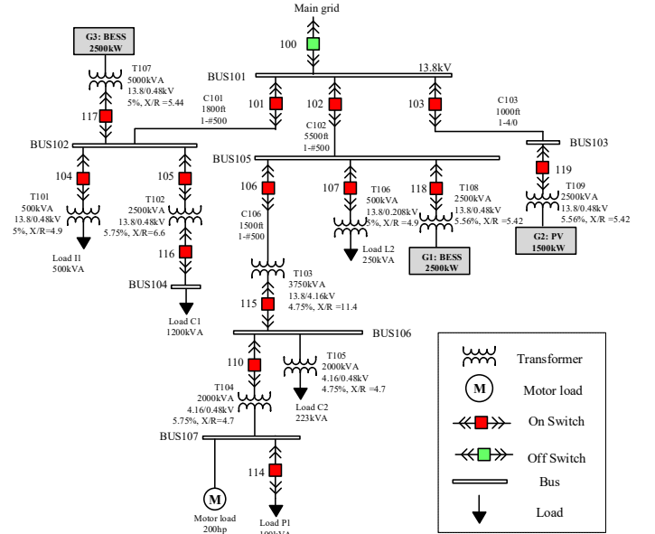
Fig. 8. Single line diagram of the islanded microgrid [28]
