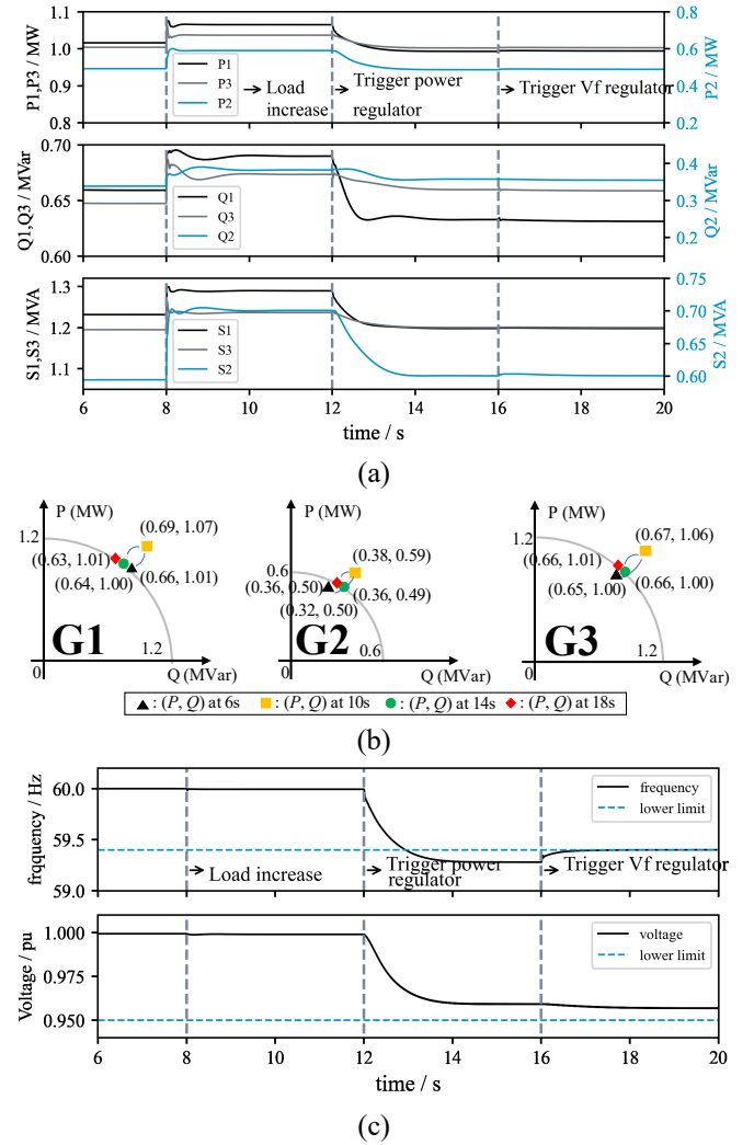
Fig. 12. Performance of the proposed control framework in Scenario 2-2: (a) dynamic inverter output; (b) static inverter output; (c) dynamic frequency and voltage
