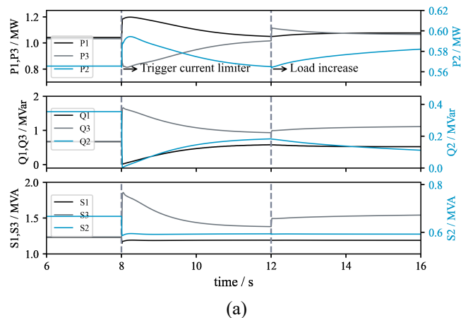
Fig. 10. Performance of current limiter in Scenario 1: (a) dynamic inverter output; (b) static inverter output; (c) dynamic frequency and voltage
